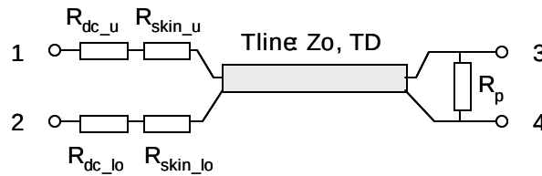
Figure 1: Lossy transmission-line grid model for power-ground plane simulations.
